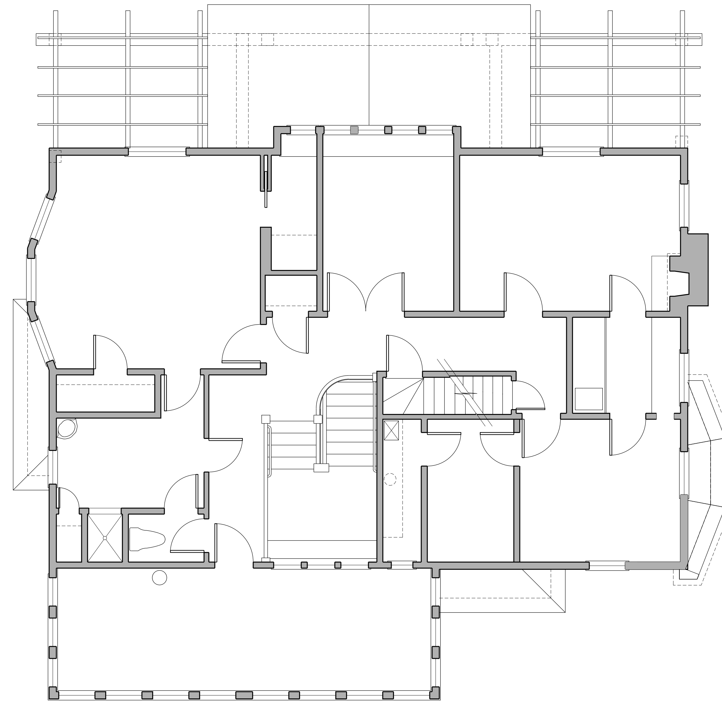
1550 SQ.FT. SECOND FLOOR
